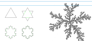
Figure 4: Left: first 4 iterations of the Koch snowflake curve. After N iterations, the length of this curve is (4/3) N
