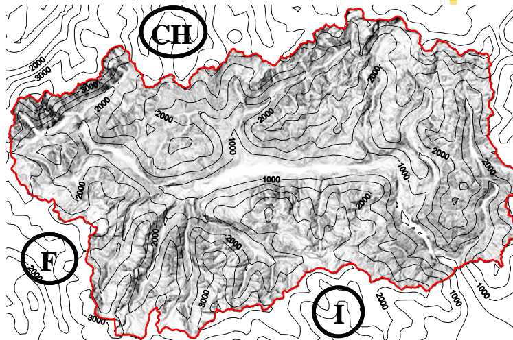
Fig. 1. Image of the Valle d'Aosta region. Boundaries (thick line) and isolines of topography levels (thin lines) are represented.
