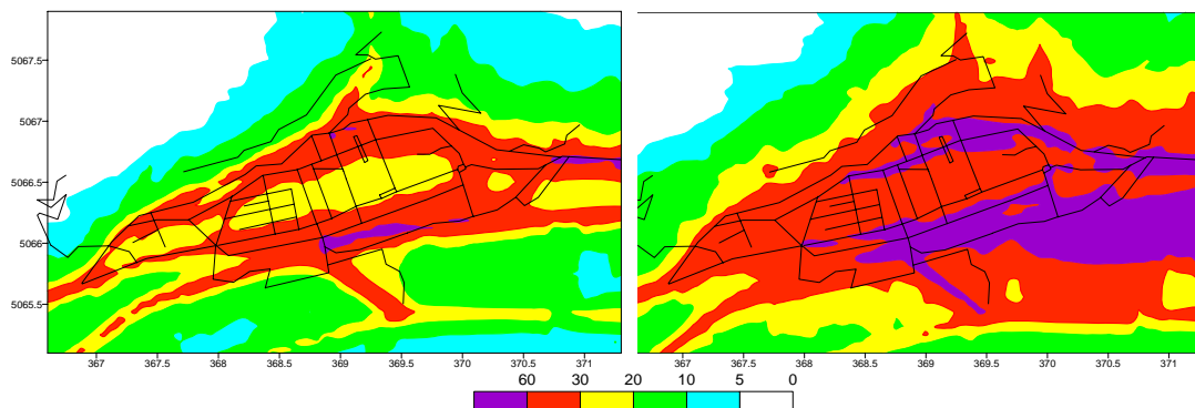
Fig. 4. NO_x annual average conc. ( \mu\text{g}/\text{m}^3 ) over Aosta town area. On the left side is represented the contribution of urban traffic emissions, while the impact of all sources is depicted on the right side.
