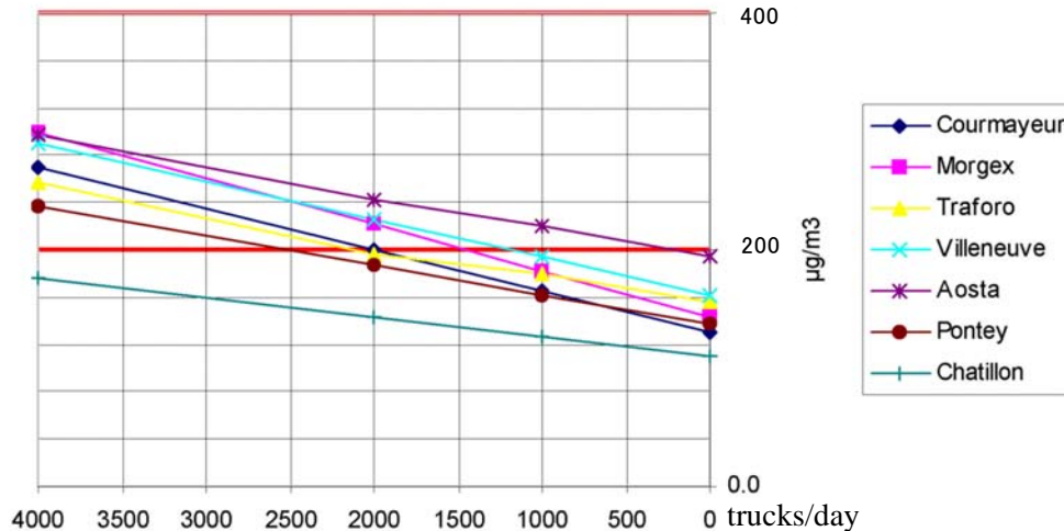
Fig. 3. Maximum annual concentration of NO 2 calculated at some sensible points close to the main road network as function of the daily number of trucks passing the Mont Blanc tunnel
