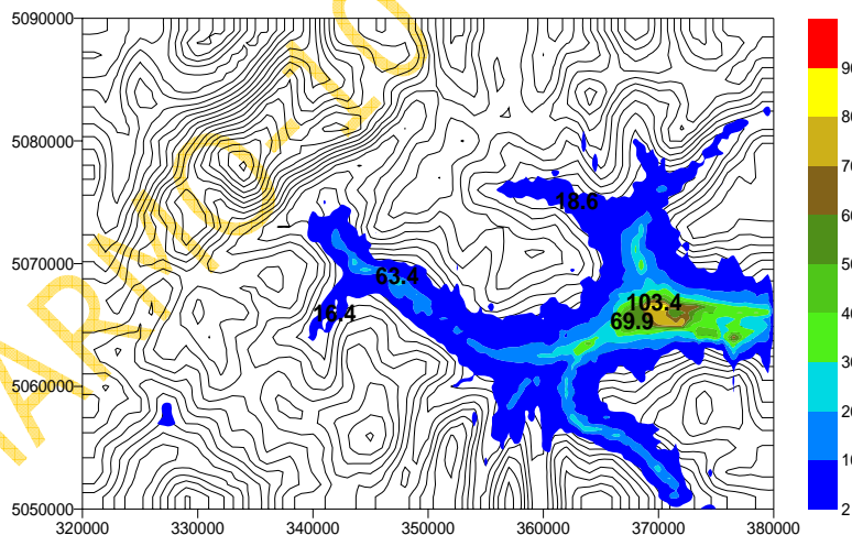
Fig. 2. Yearly average ground level concentration map of NO x for year 2001. Values are in \mu\text{g}/\text{m}^3 . Numbers represent annual averages measured by the local network.
