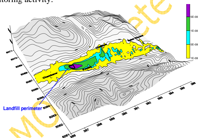
Fig 5. Map of the annual mean dilution factor due to an emission from the area of the landfill.
