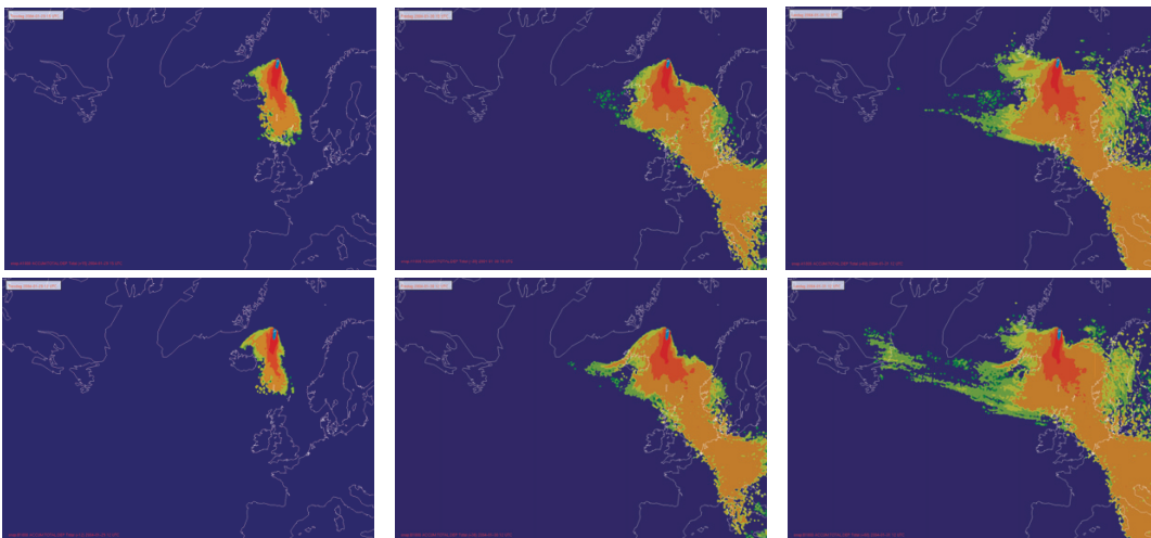
Figure 4. Comparison of accumulated total deposition for cylinder (upper) and mushroom (lower) initial shapes for the radioactive cloud: 12, 36, and 60 hrs after the explosion. The location of explosion is Jan Mayen and the yield is 1000 ktonnes.
