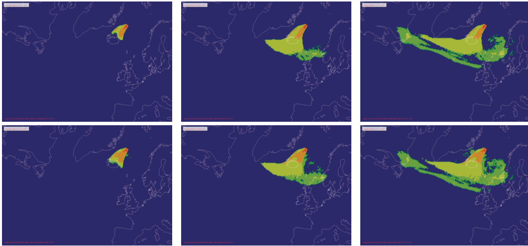
Figure 3. Comparison of accumulated total deposition for cylinder (upper) and mushroom (lower) initial shapes for the radioactive cloud: 12, 36, and 60 hrs after the explosion. The location of explosion is Jan Mayen and the yield is 10 ktonnes.
